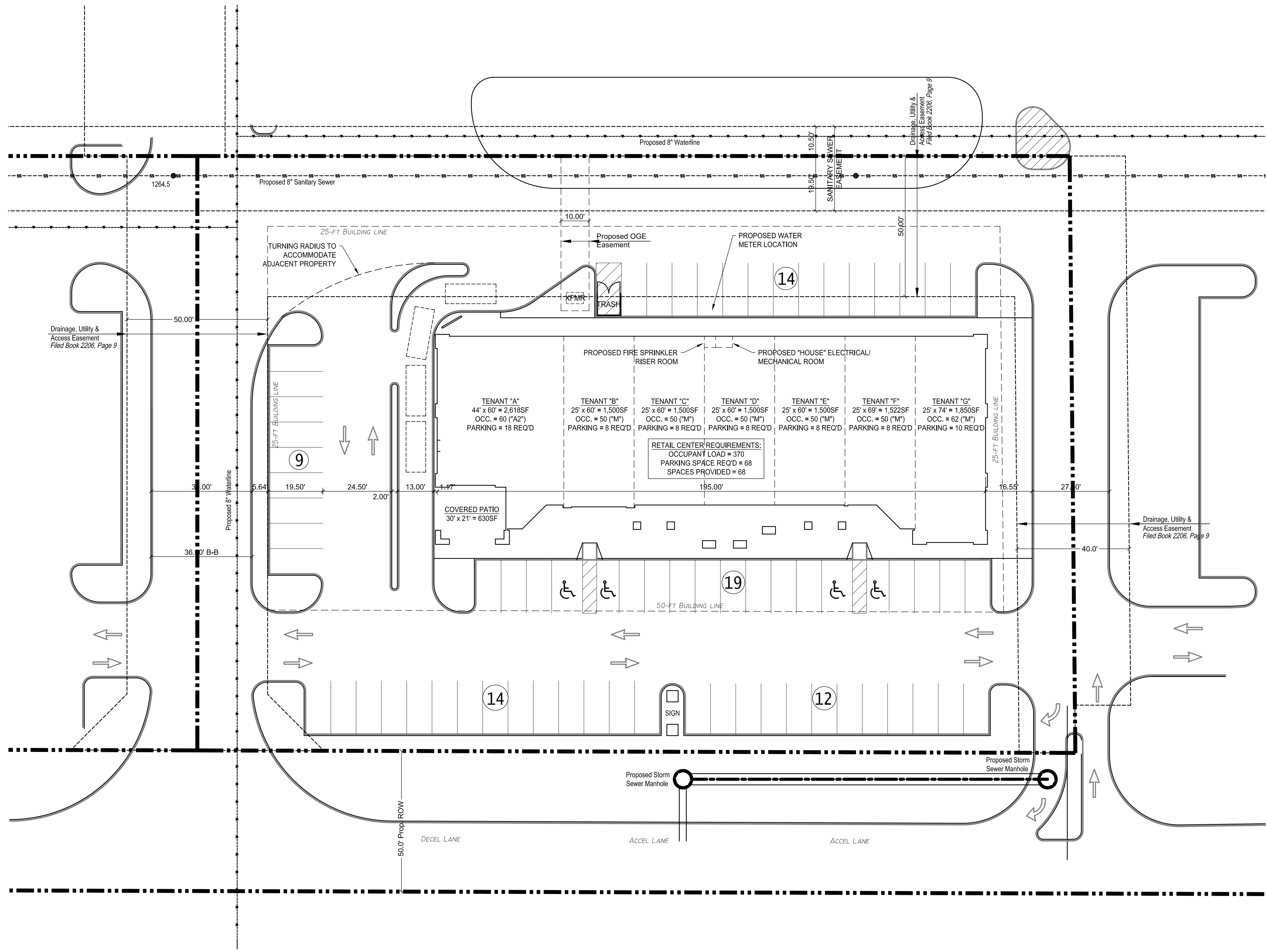
1 SITE PLAN 1" = 20'-0"
